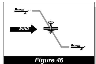
Effect of wind and forward inertia on flight path during one turn spin (effect exaggerated)
