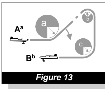
Family 1.12-1.19 as flown. Radii a, b, and c may all be different and entrance altitude "A" can be different from exit altitude "B".
